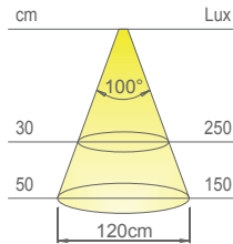
values referring to FLEXYLED SE H4-24 D-M 1000mm
